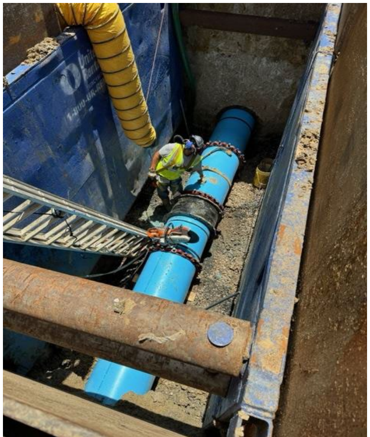
24" Gravity Sewer Replacement Pipe
