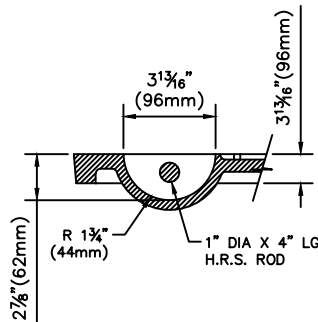
PICKBAR DETAIL
