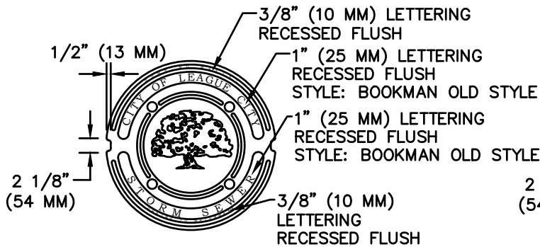
COVER PLAN VIEW
