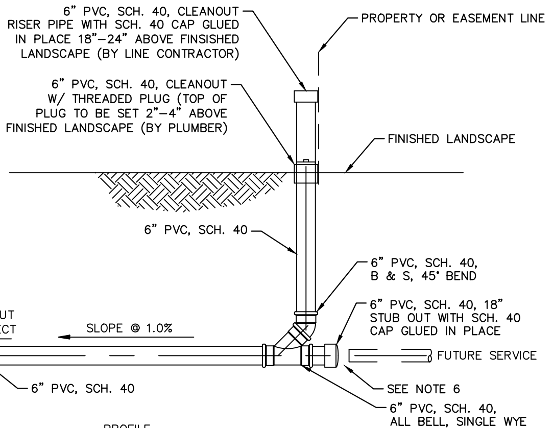
PROFILE
