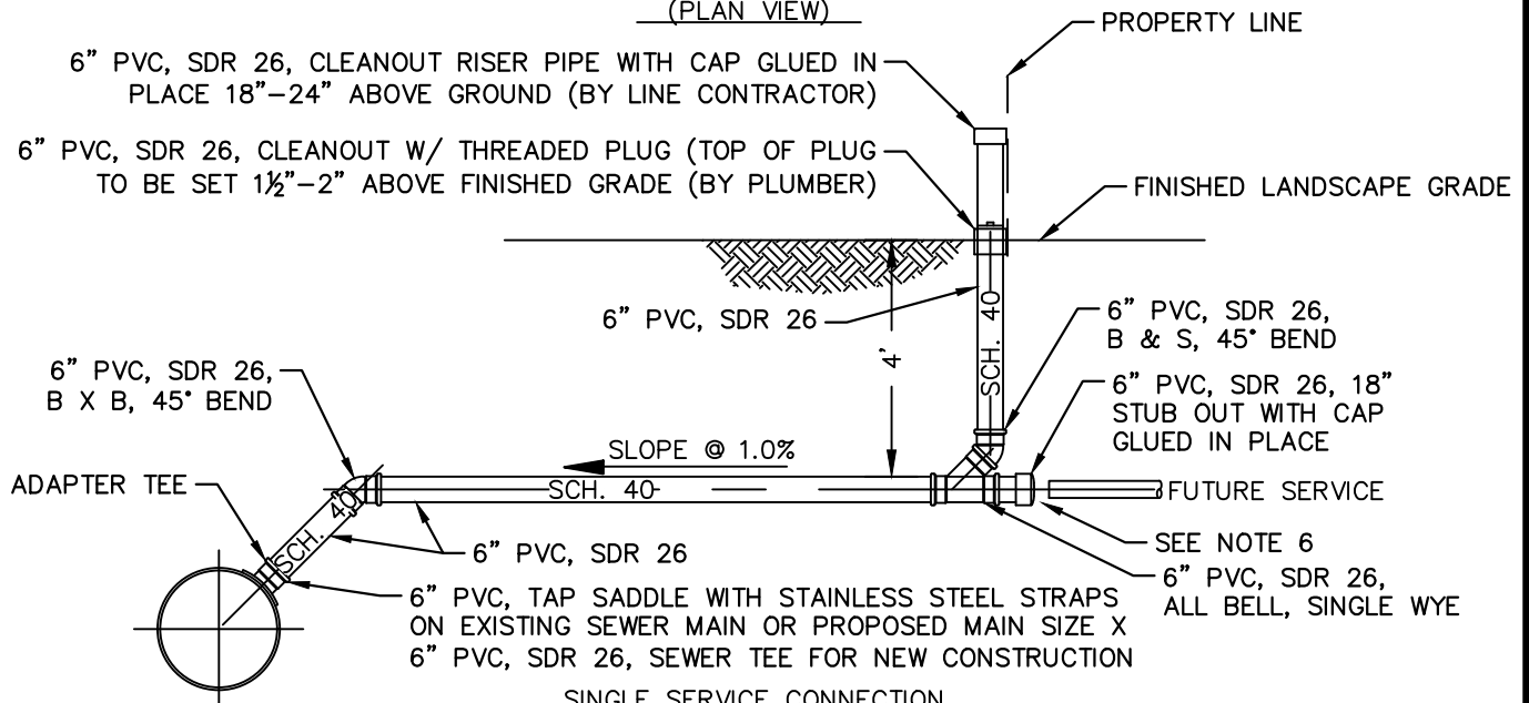
SINGLE SERVICE CONNECTION (PLAN VIEW)
