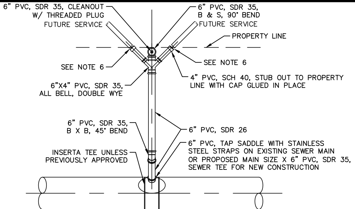
DOUBLE SERVICE CONNECTION (PLAN VIEW)
