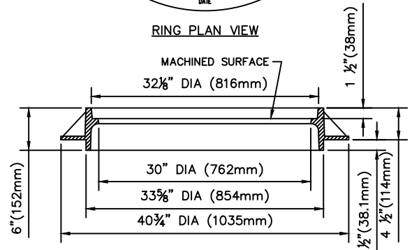
RING CROSS SECTION
