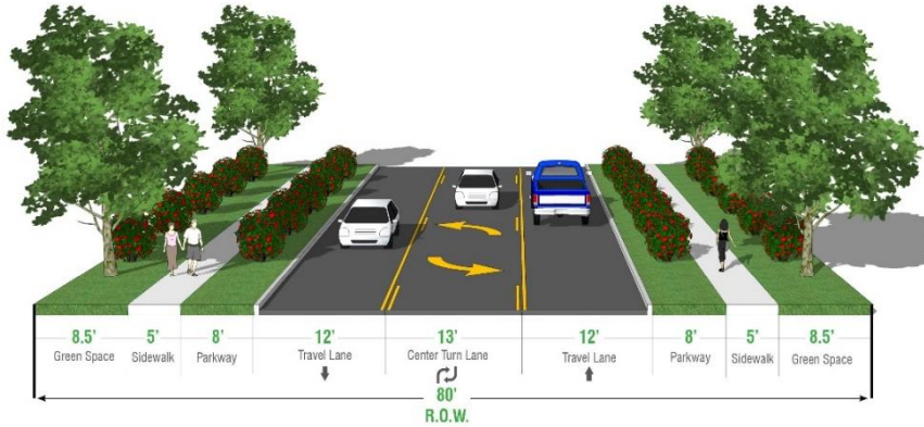
Figure 9. Collector - 3 Lanes, 80' ROW, 12- Foot Lanes
