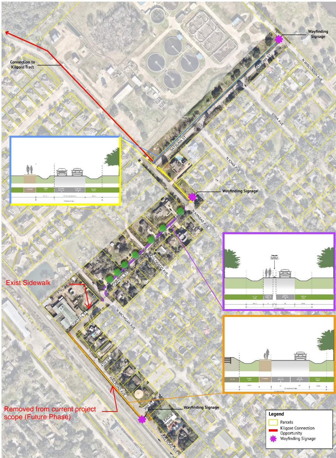
Figure 8 – Preferred Alignment with Cross Sections
