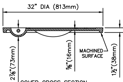
COVER CROSS SECTION
