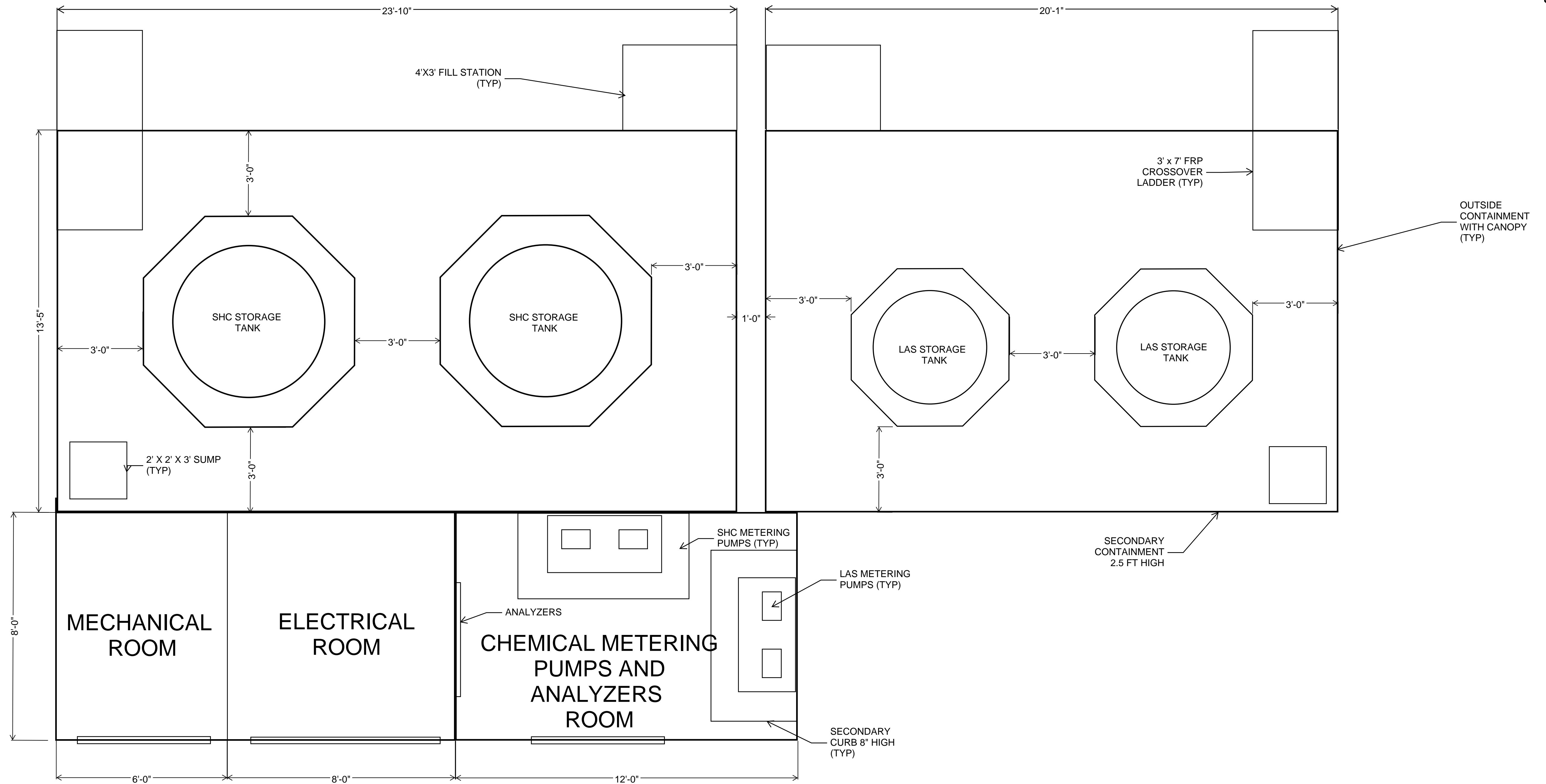
PLAN 1/2" = 1'0"
